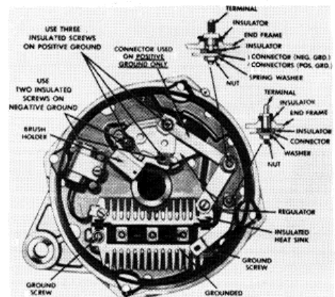
27-SI Series 200 Type (Stator, Diode Trio, and One Insulating Screw Removed)
