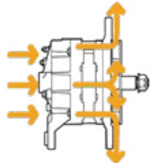
Conventional External Single Fan
